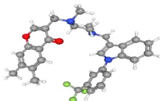
Gambar 4. Struktur TNF-alfa Inhibitor
